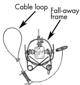
Figure BC20a. Powered cable device
