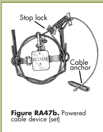
Figure RA47a. Powered cable device
